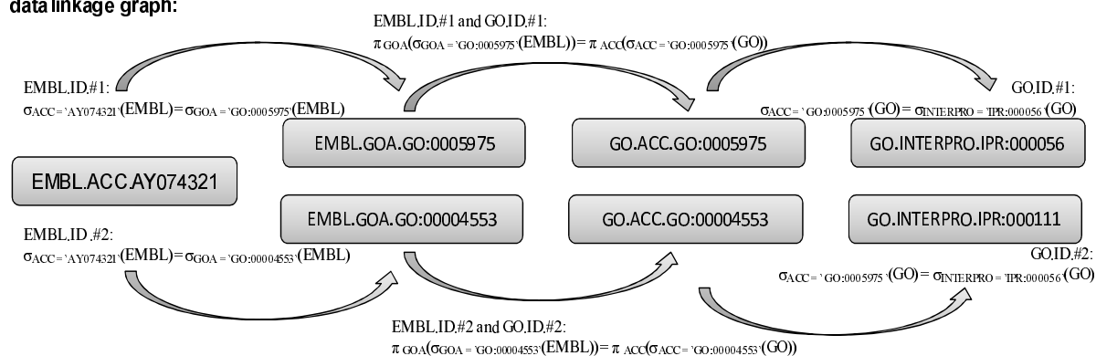
Figure 1: example for the relationships in schema and data linkage graphs
