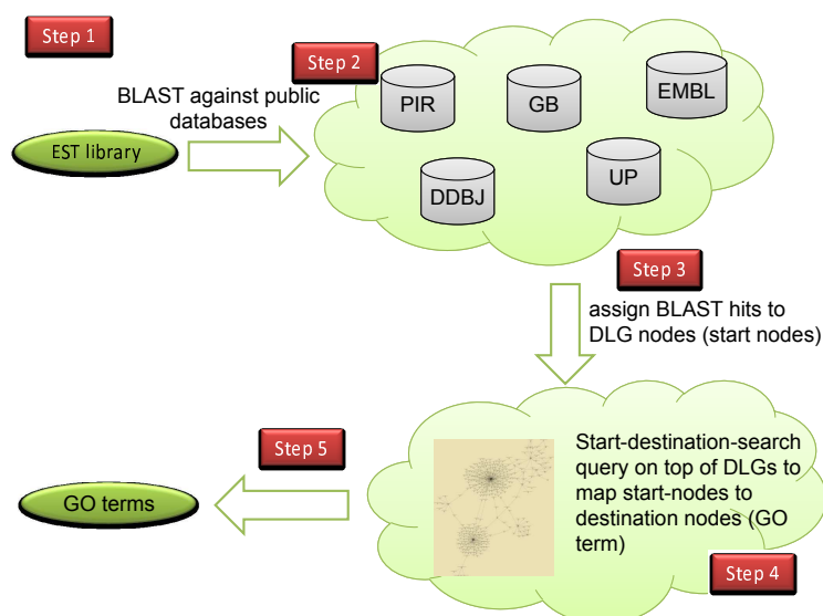
Figure 2: work flow to assign ESTs to GO terms
