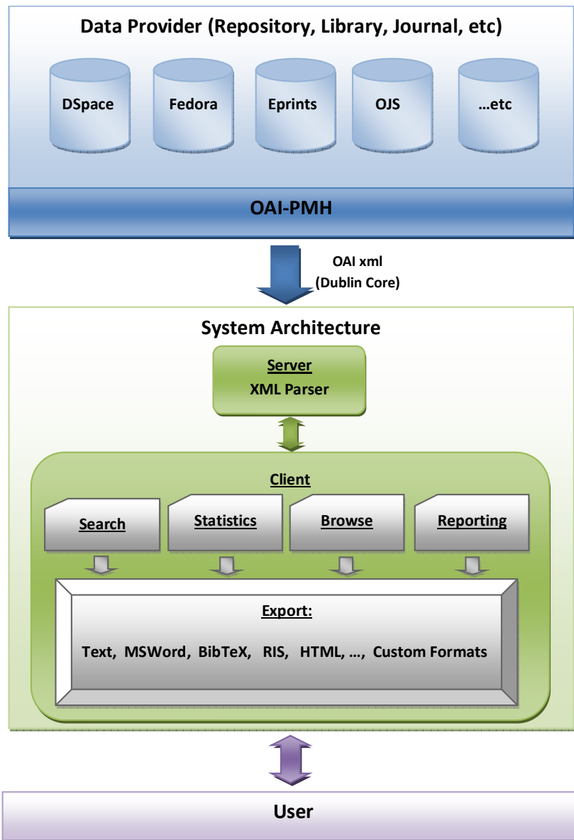
Figure 1. Architecture of value-added service implementation.
