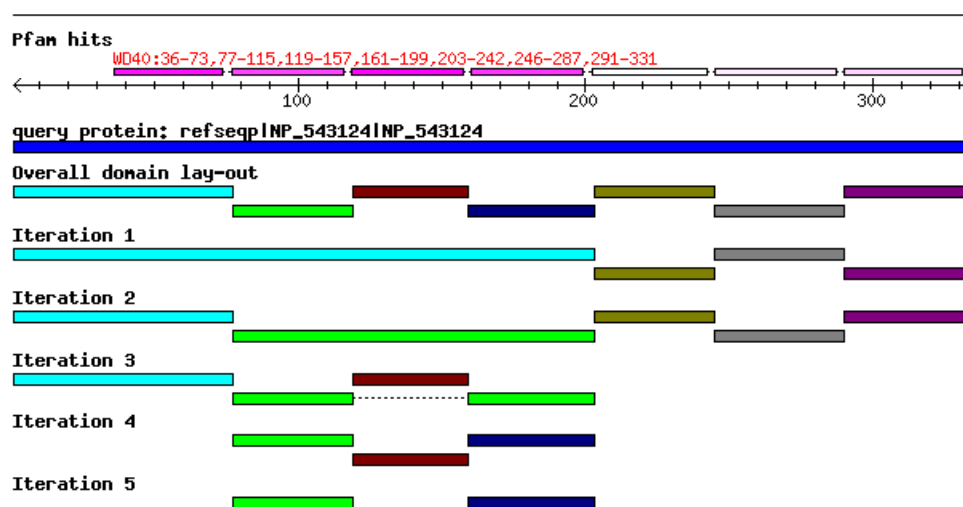
Figure 3: The domain lay-out of WDR5 as present on the web output. Above the query protein (blue) the Pfam hits (repeats and domain classes) are shown. As these seven hits are from the same Pfam family, they are presented in one track. The track “Overall domain lay-out” summarizes all domains found in all DOMAINATION iterations. Domains are coloured based on the start position of the domain and numbered per iteration. This is followed by the results per iteration. Each domain formed during an iteration is used in the next iteration. Domains that are not split again are not used in the next iteration ( e.g. the last three domains in iteration 2).
