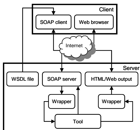
Figure 1: The tool specific WSDL file is used by the user to produce the SOAP client, which sends a request to the remote SOAP server. This request is forwarded to the respective tool via a wrapper. The SOAP server processes the tool's output and sends back the results or a ticket, which can be polled until the tool run has been completed. For several tools, the result also contains a URL. In these cases, the output is also available as an interactive HTML web page, which can be viewed in the user's web browser.
