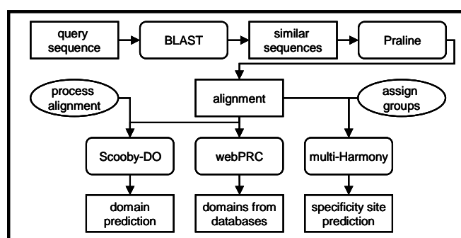
Figure 2: Example workflow. A query sequence is BLASTed and hits are extracted. These sequences are aligned with the Praline service. The alignment can then be used for three other tools: Scooby-Domain, webPRC and multi-Harmony. For Scooby-Domain, the alignment may need to be pre-processed ("process alignment", cf. [8]). Before multi-Harmony can be used, the sequence groups need to be assigned first ("assign groups").
