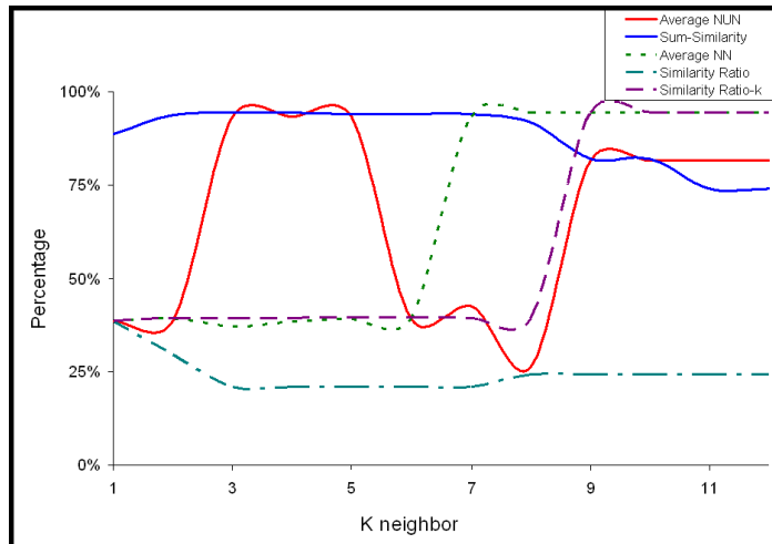
Fig. 5. The five predictors are compared in order to set a confidence threshold.
