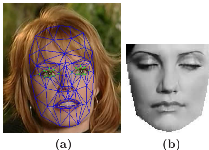
Fig. 1. (a) The 3D mesh is projected onto the input image I_t in order to construct the appearance model \mathbf{A}_t by a warping process (b).
